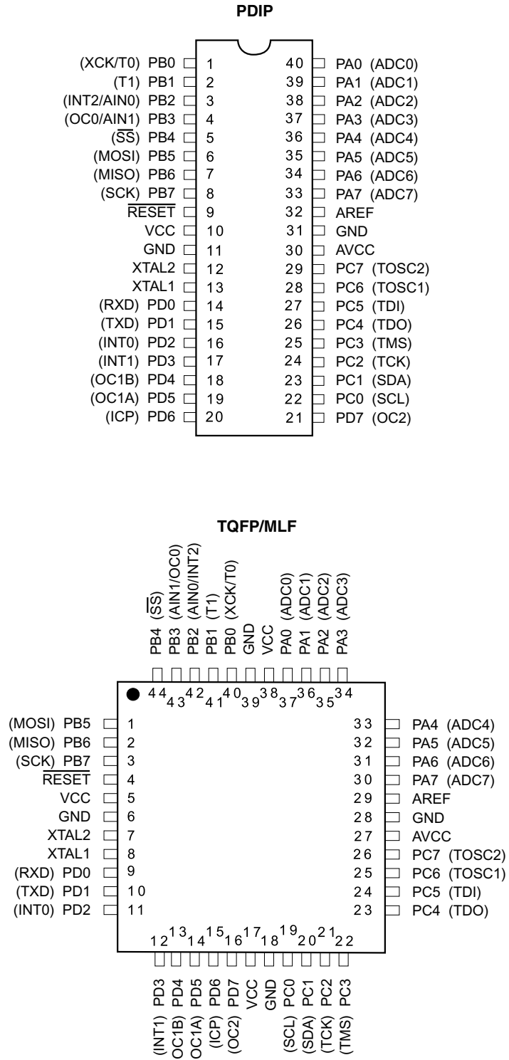
Figure 1. Pinouts ATmega16
